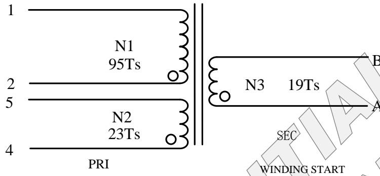
Figure 4: Transformer Diagram
